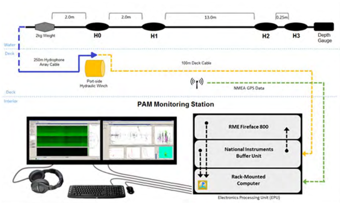
Figure 3: Simplified pathway of data through the PAM system on board the Langseth.
