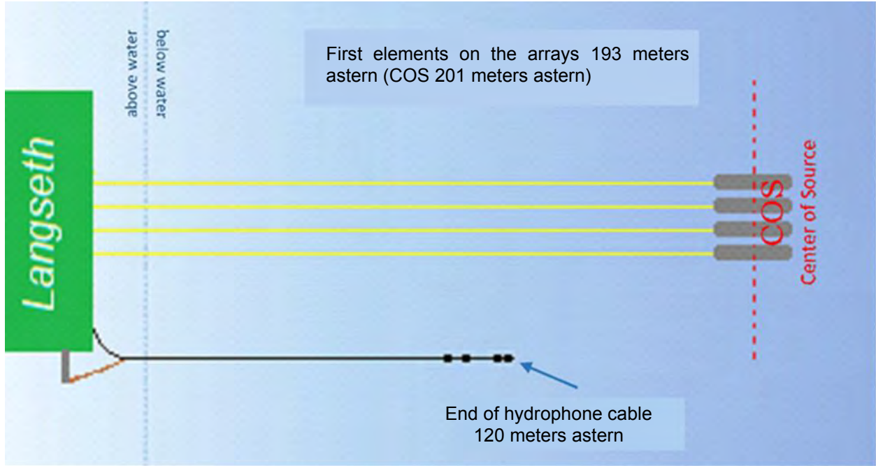
Figure 4. Location of the PAM cable in relation to the seismic gear during the seismic survey.
