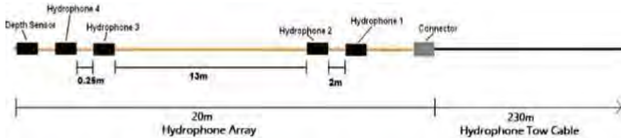
Figure 8: Two-part hydrophone cable with a 230-meter tow cable and detachable 20-meter hydrophone array
