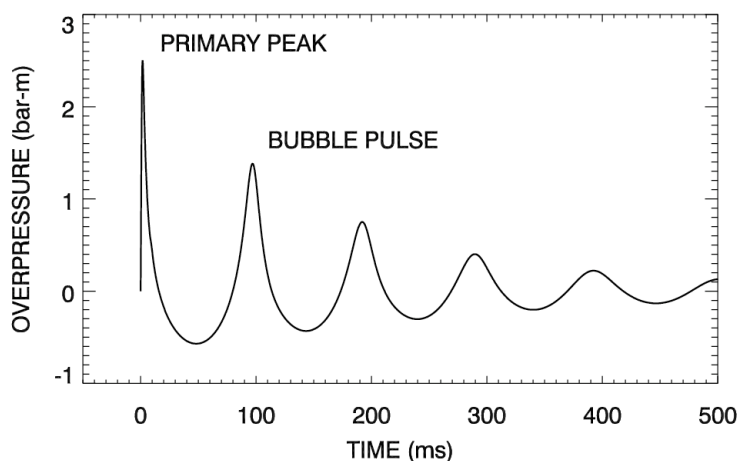
FIGURE B. 1: Overpressure signature for a single airgun, showing the primary peak and the bubble pulse.
