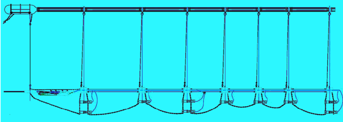
FIGURE 2. One linear airgun array or string.
