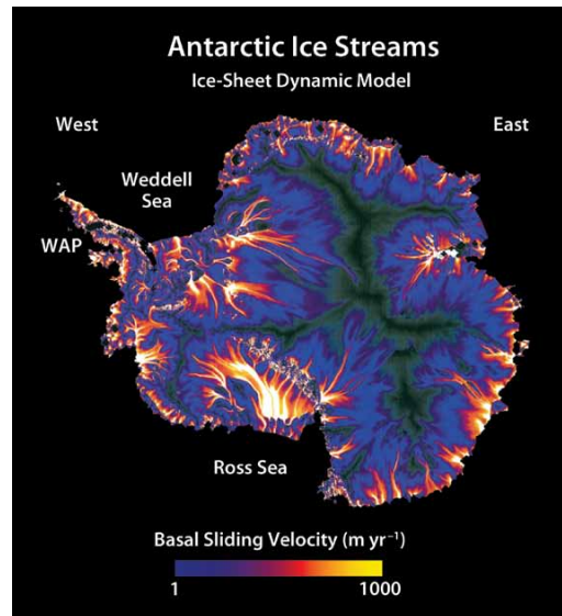
Figure 4.74. Antarctic ice sheet drainage. Source: Snowball Earth.
