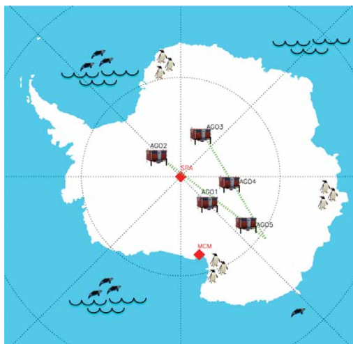
Figure 3.14. Map of Automatic Geophysical Observatory locations. Observatory components are aligned along geomagnetic longitudes that converge at the geomagnetic south pole. Source: Siena College and New Jersey Institute of Technology.
