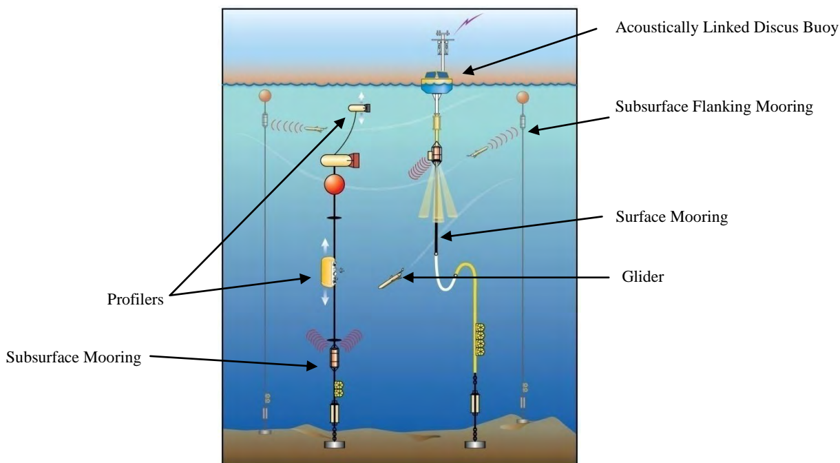
Figure 2-13 Representation of an Acoustically Linked Disc Buoy and Subsurface Moorings Proposed for Use at the High-Latitude GSN Sites
