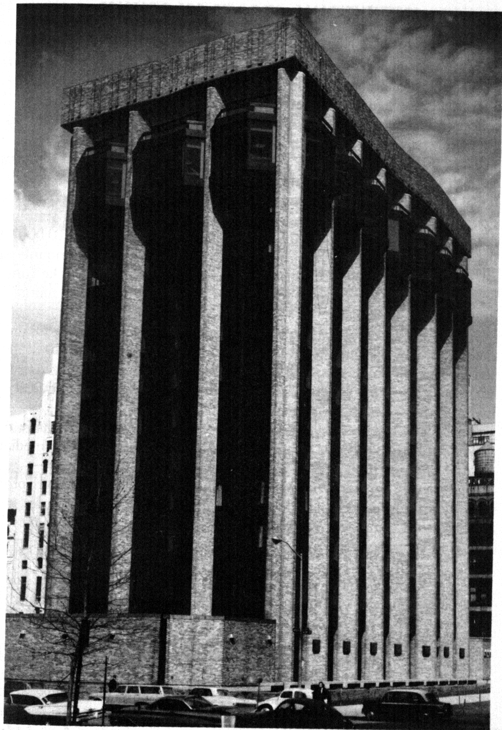
Figure 36.—Warren Weaver Hall of the New York University.
