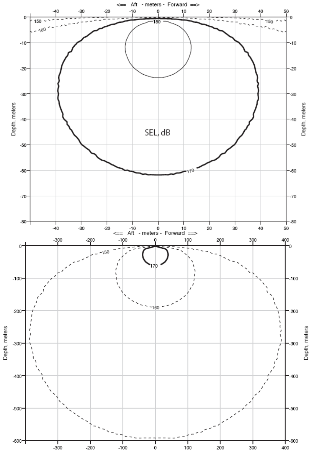
FIGURE 3. Modeled received sound levels (SELs) in deep water from a single 40-in 3 airgun, which is planned for use as a mitigation airgun during the survey in the central Pacific Ocean, 26 November–29 December 2011. Received rms levels (SPLs) are expected to be ~10 dB higher.
