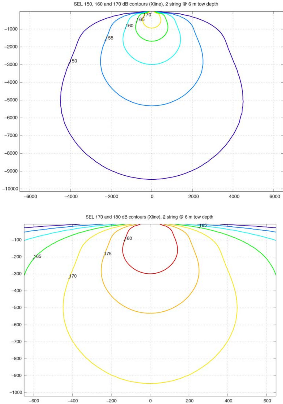
FIGURE A3. Deep-water model results for the 18-gun, 3300-in 3 , 2-string array at 6-m tow depth, the configuration that was used to collect calibration measurements presented in Figure 2. The 150-dB SEL, 170-dB SEL, and 180-dB SEL distances can be read at 4500 m, 450 m, and 142 m.
