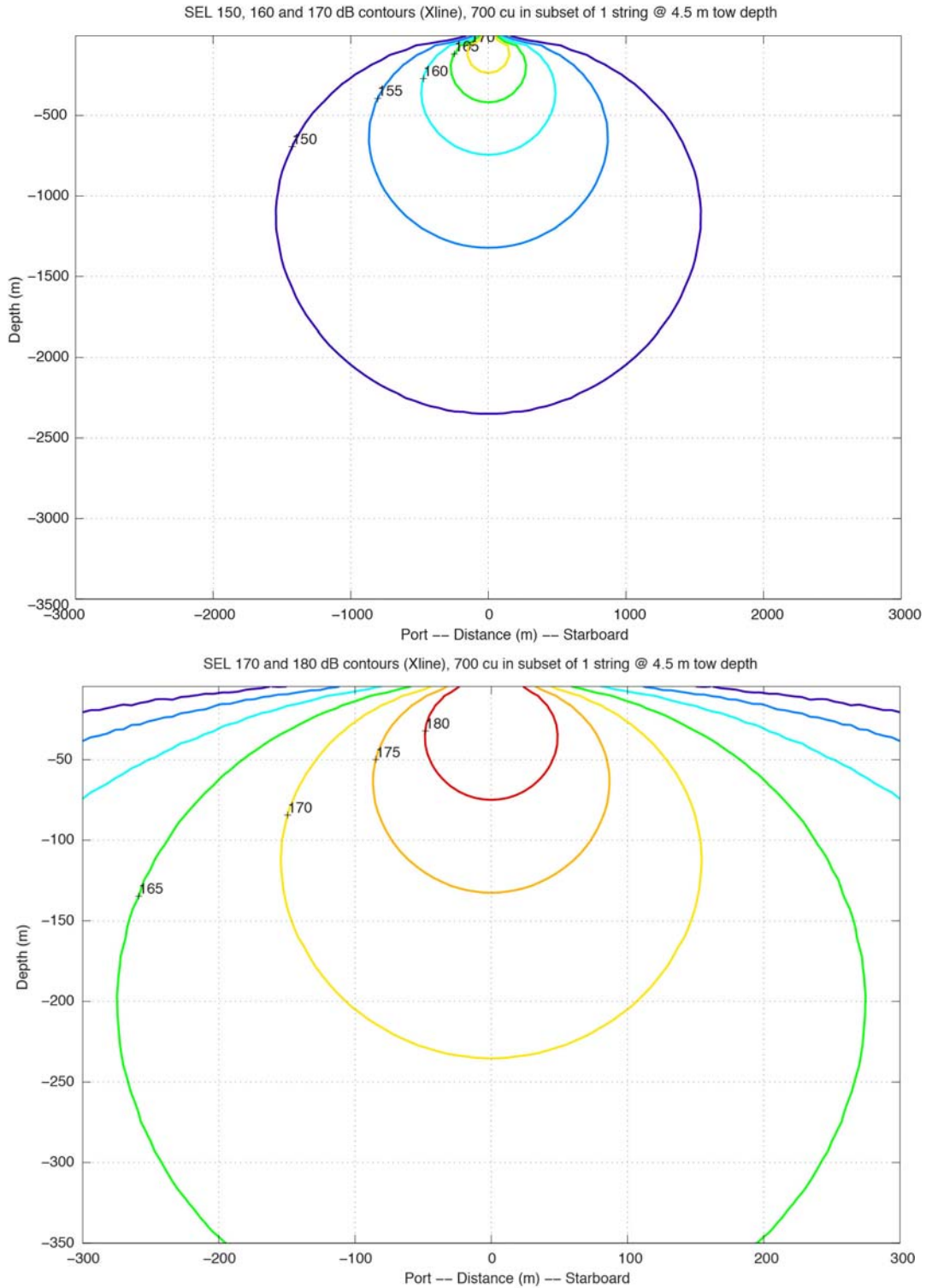
FIGURE A4. Deep-water model results for the 4-gun, 700-in 3 subset of 1-string array at 4.5-m tow depth that could be used for the NJ margin 3D survey. The 150-dB SEL, 170-dB SEL, and 180-dB SEL distances can be read at 1544 m, 155 m, and 49 m, respectively.
