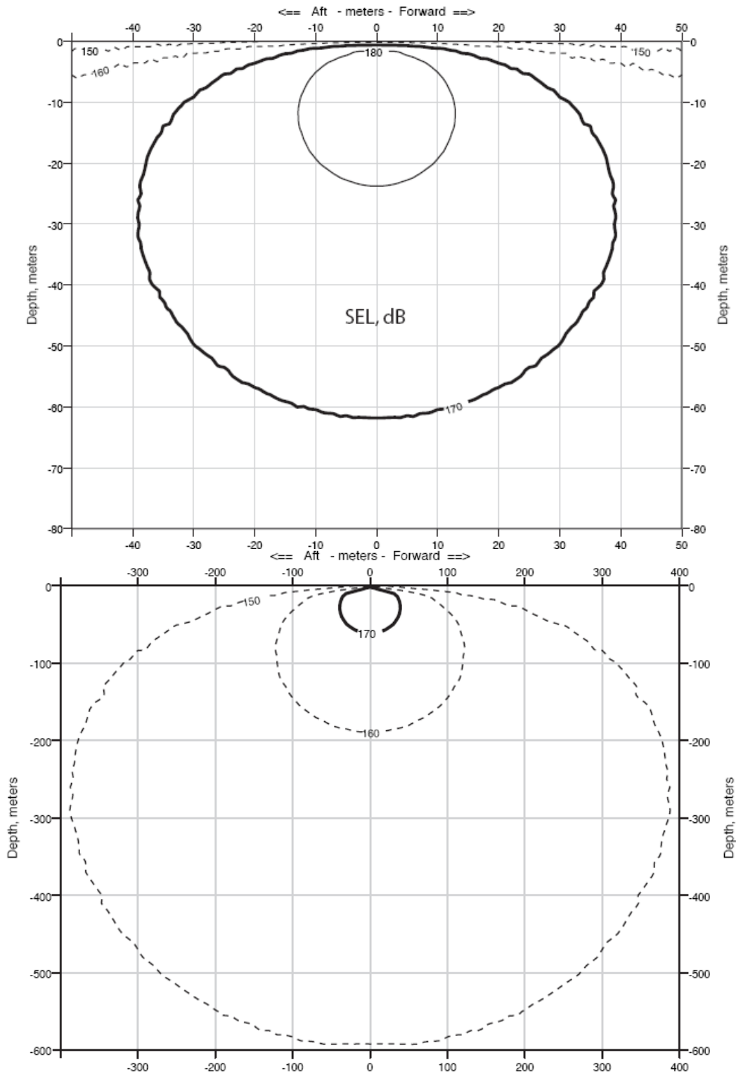
FIGURE 3. Modeled received sound levels (SELs) from a single 40-in 3 airgun operating in deep water, which is planned for use as a mitigation airgun during the Shatsky Rise survey, 17 June–31 July 2010. Received rms levels (SPLs) are expected to be ~10 dB higher.
